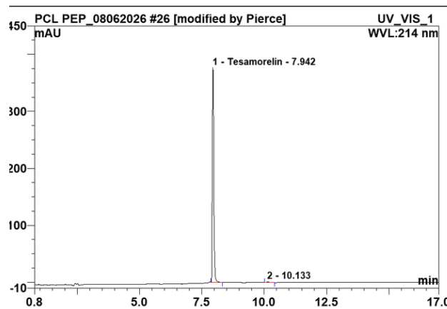
HPLC Chromatogram (Retention Time: 7.94 min)
