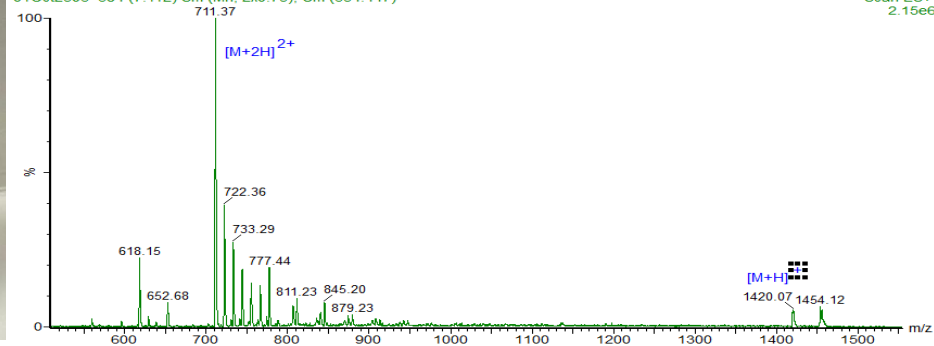
BPC-157 500mcg, IG-87 QC251367B, Conc'd 01Oct2503 384 (7.112) Sm (Mn, 2x0.75); Cm (354.447)
